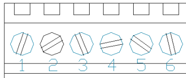
Figure 13: RS422 Header
