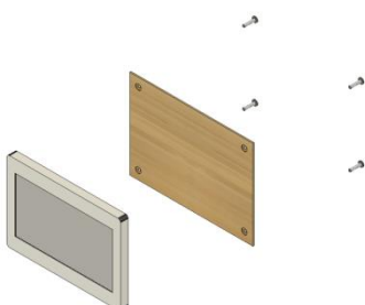
Figure 17: Display Assembly Installation
