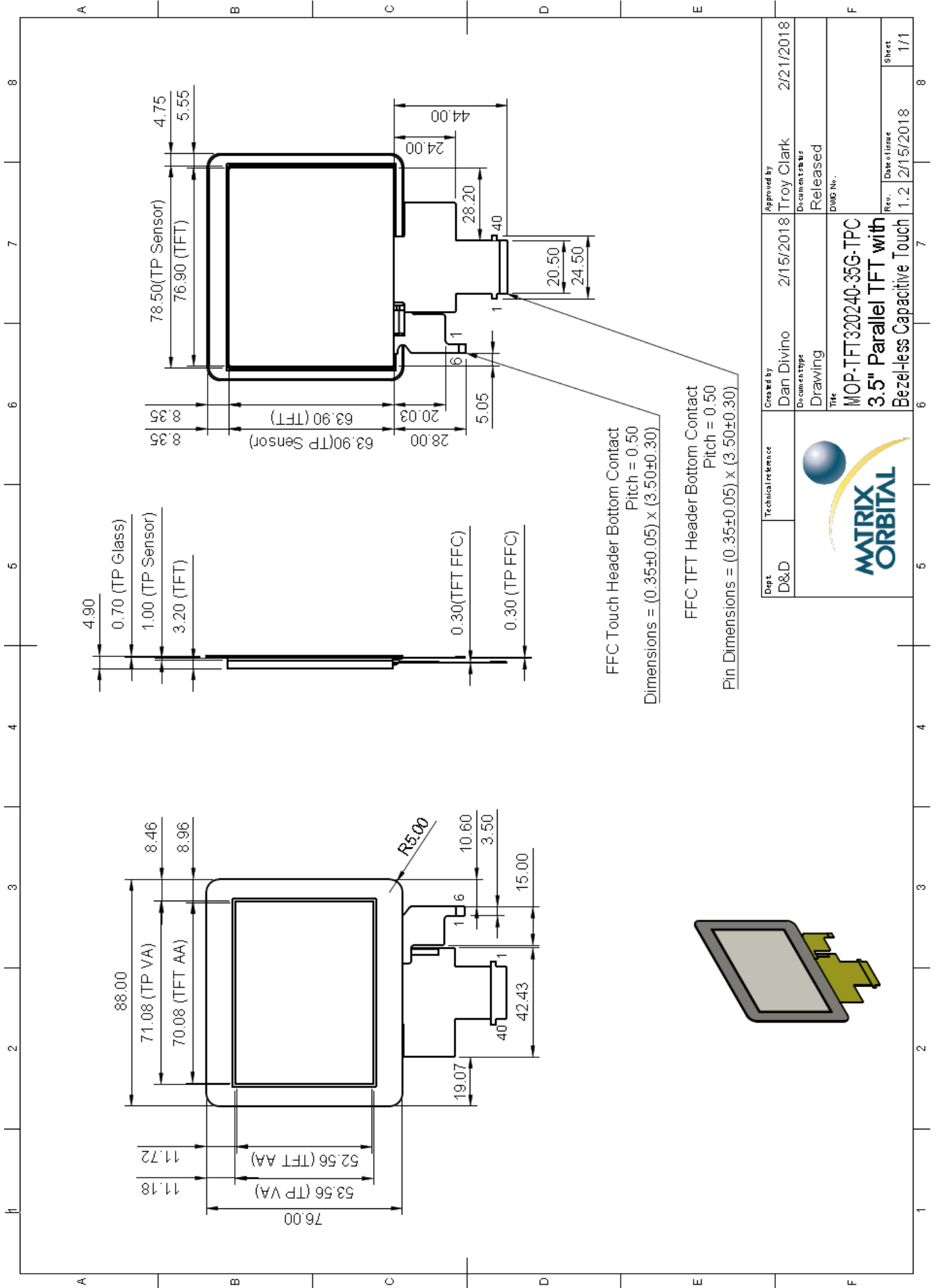
Figure 1: MOP-TFT320240-35G-BLM-TPC Drawing
