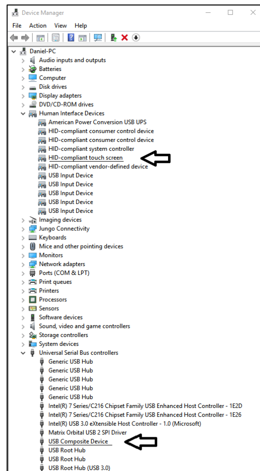
Figure 9: HTT USB Driver Listing
