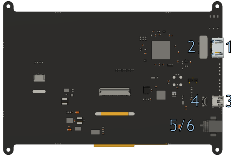
Figure 2: HTT70A Headers
