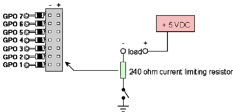
Figure 2-8 General Purpose Outputs
