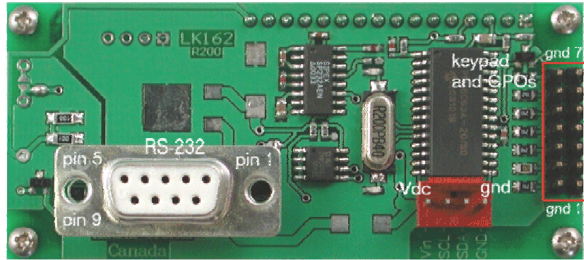
Figure 2-1 Electrical Connections
