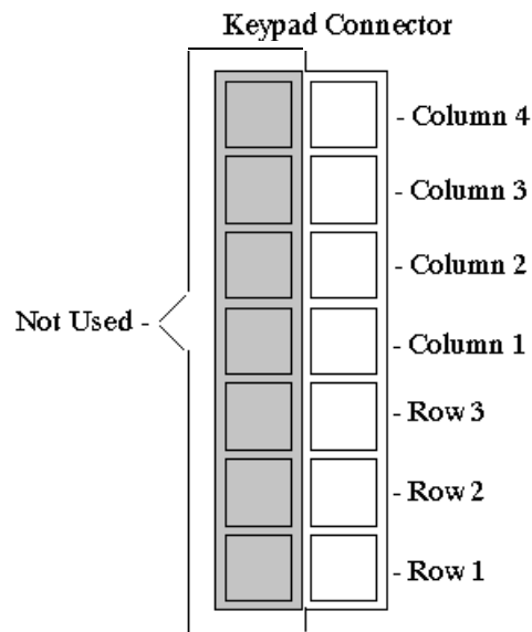
Figure 4-1 Keypad Connector
