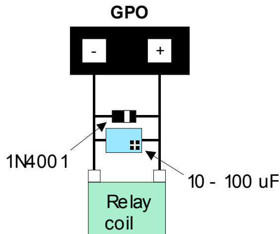
Figure 2-9 Clamping a Relay
