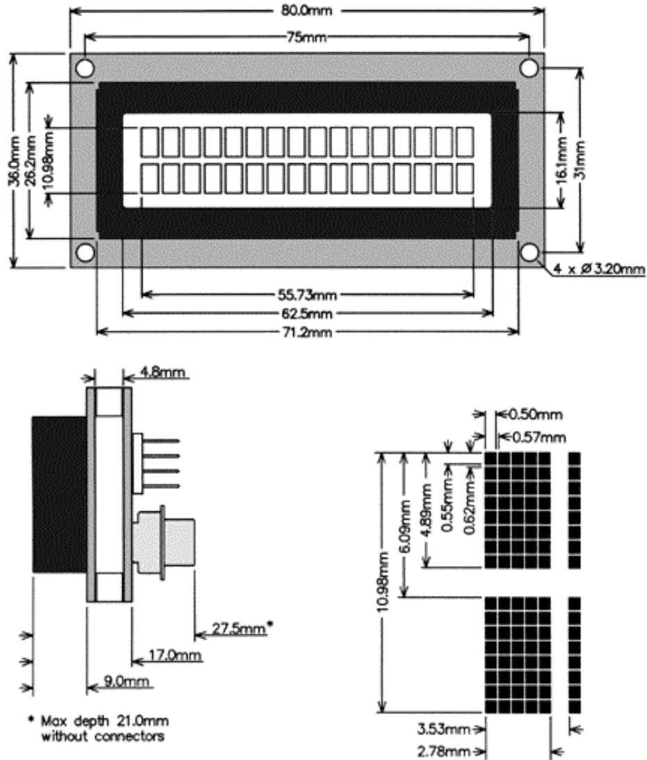
Figure 8-1 Physical Layout
