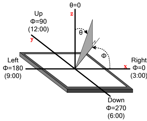
Figure 2: The definition of viewing angle
