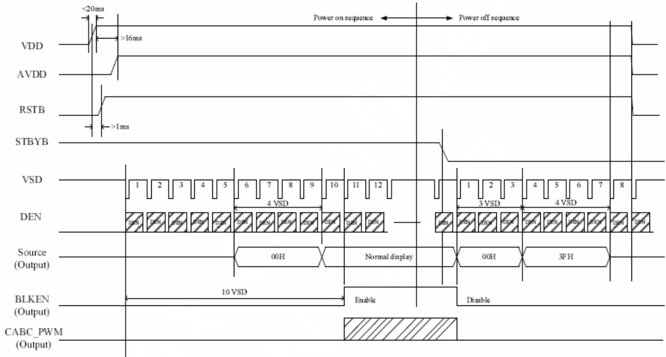
Figure 7: Power up sequence timing diagram
