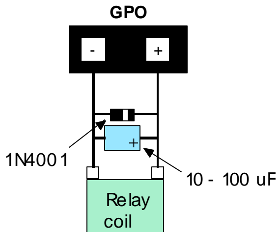
Figure 2-9 Clamping a Relay
