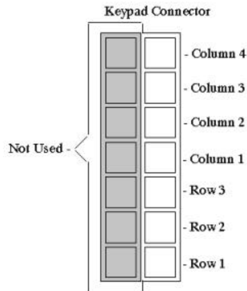
Figure 4-1 Keypad Connector
