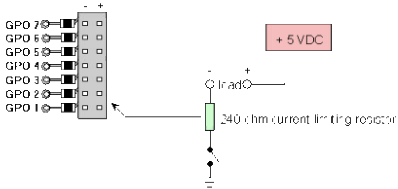
Figure 2-8 General Purpose Outputs
