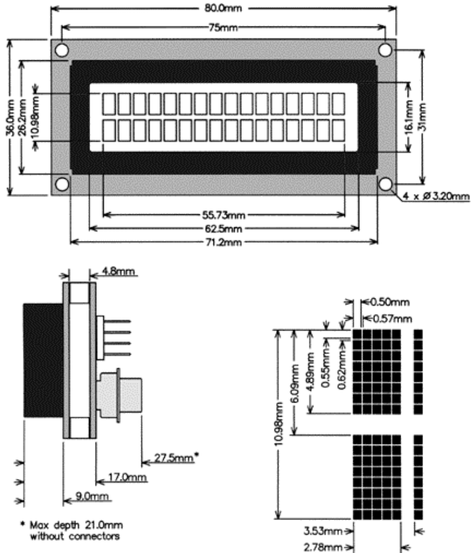
Figure 8-1 Physical Layout
