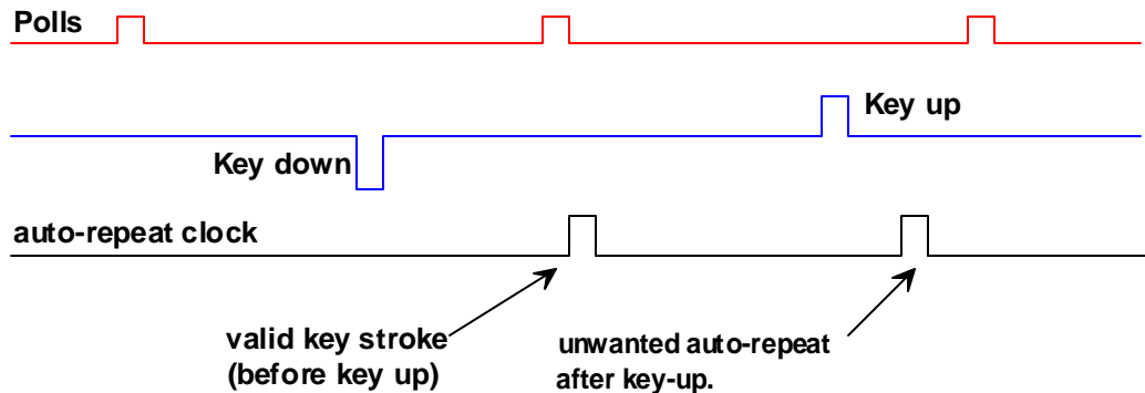
Figure 4-2 Poll timing
