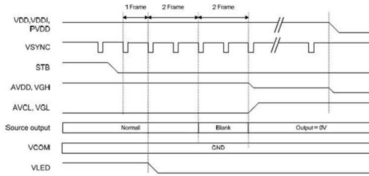
Figure 2: Power Down Sequence
