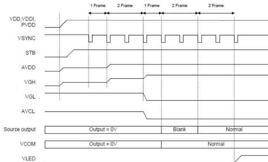
Figure 1: Power Up Sequence
