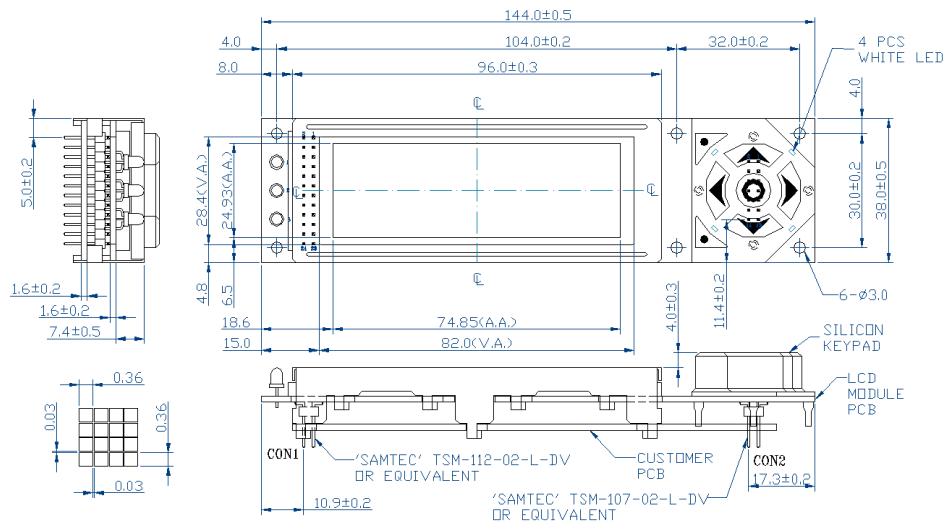
Figure 1: MOP-GL19264R Mechanical Drawing
