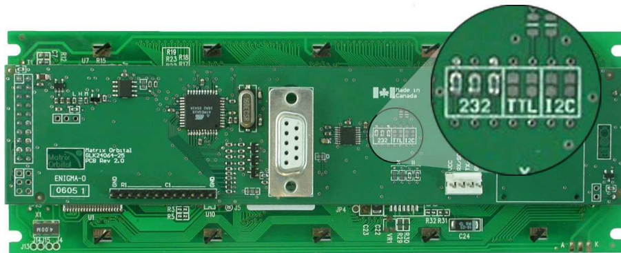
Figure 19: Protocol Select Jumpers
